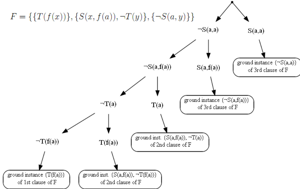
Figure 2: A closed semantic tree for F .
